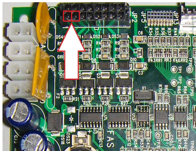
Detail of connector JP2
